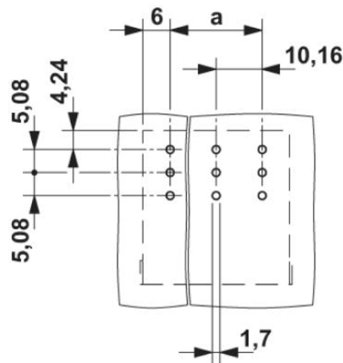
Drilling diagram
