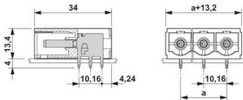
Dimensioned drawing
