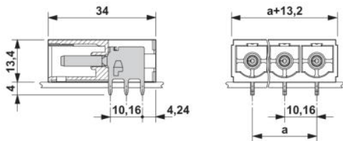
Dimensioned drawing
