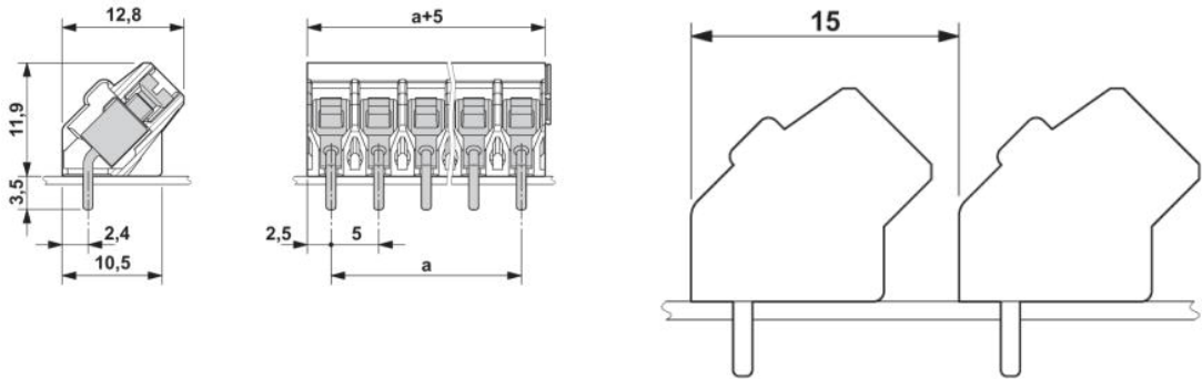
Dimensioned drawing
