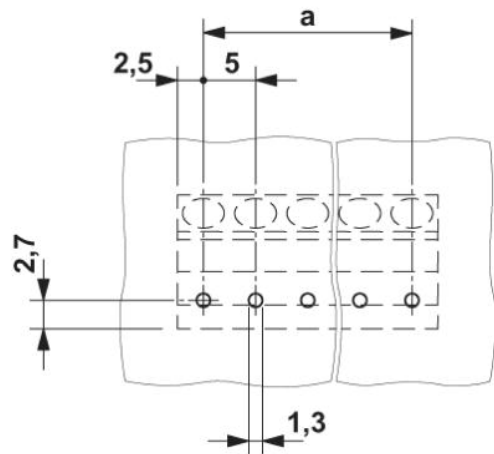
Drilling diagram
