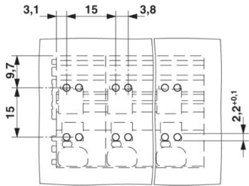
Drilling diagram
