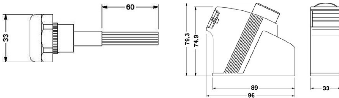
Dimensioned drawing
