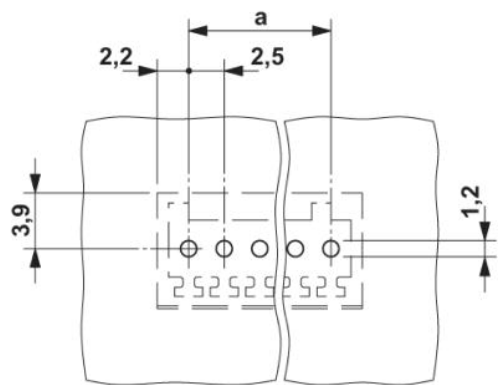
Drilling diagram
