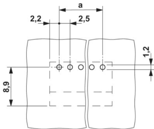
Drilling diagram
