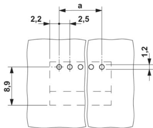
Drilling diagram
