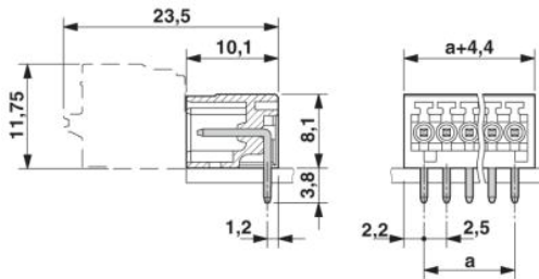
Dimensioned drawing
