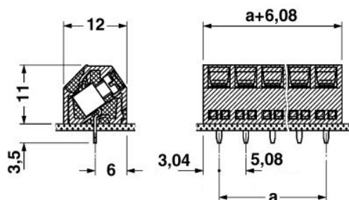
Dimensioned drawing
