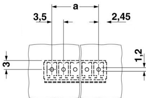
Drilling diagram
