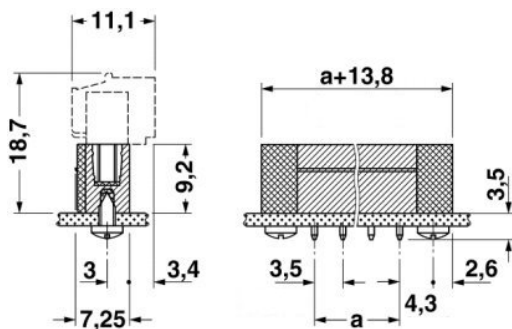
Dimensioned drawing
