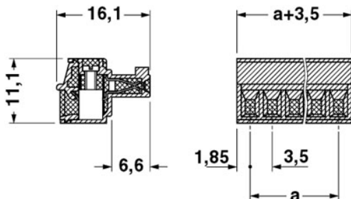
Dimensioned drawing
