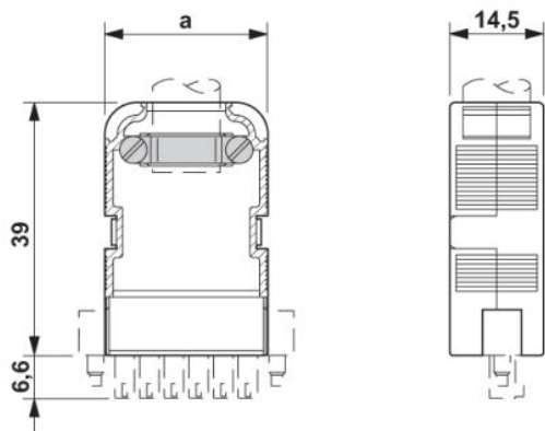
Dimensioned drawing
