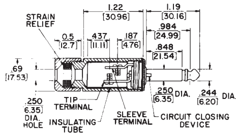
2-Conductor "Silent Plug", No. 172
