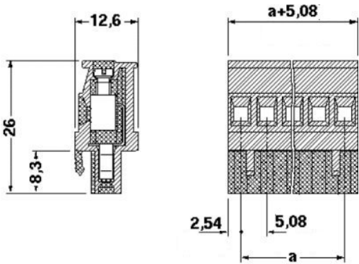
Dimensioned drawing
