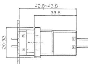
Panel/Free-Hanging Type
