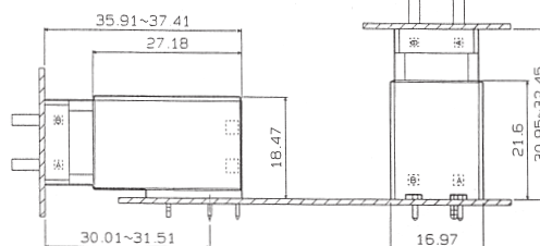
Horizontal/Vertical Type
