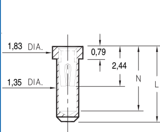
XXXX-0-15-XX-30-XX-10-0 Solder mount in 1,4 min. mounting hole
