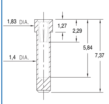
8363-0-15-XX-35-XX-10-0 Solder mount in 1,45 min. mounting hole
