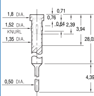
3018-0-15-XX-30-XX-04-0 Press-fit in 1,45 mounting hole
