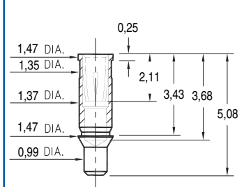
1385-0-15-XX-43-XX-10-0 Surface mount
