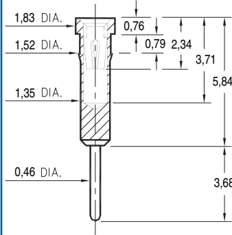
4001-0-15-XX-43-XX-04-0 Press-fit in 1,45 mounting hole
