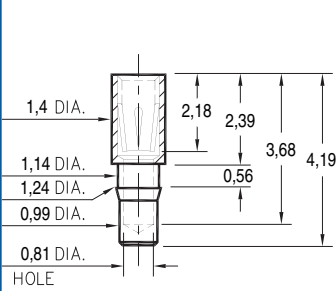
0385-0-15-XX-43-XX-10-0 Press-fit in 1,17 mounting hole
