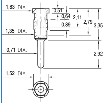
5960-0-15-XX-43-XX-04-0 Hex press-fit in 1,45 plated thru hole
