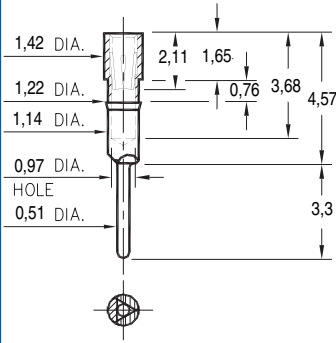
1782-0-15-XX-43-XX-04-0 Press-fit in 1,14 mounting hole
