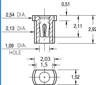
3907-0-18-XX-30-XX-10-0 Surface mount Also available on 12mm wide carrier tape: 4,000 parts per 330mm reel. Order as: 3907-0-58-XX-30-XX-10-0
