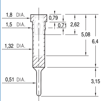
8852-0-15-XX-30-XX-04-0 Press-fit in 1,42 mounting hole
