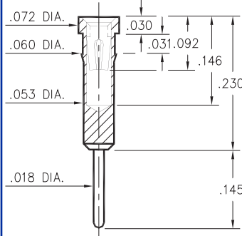
4001-0-15-XX-43-XX-04-0 Press-fit in .057 mounting hole
