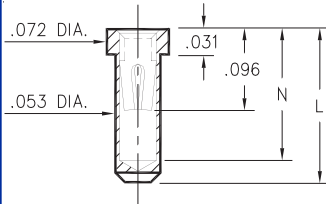
XXXX-0-15-XX-30-XX-10-0 Solder mount in .055 min. mounting hole
