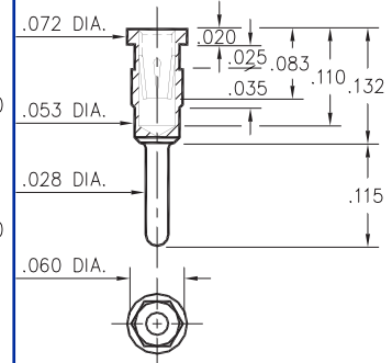
5960-0-15-XX-43-XX-04-0 Hex press-fit in .057 plated thru hole
