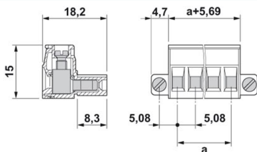
Dimensioned drawing
