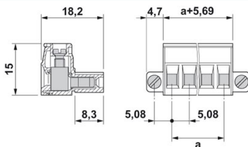
Dimensioned drawing
