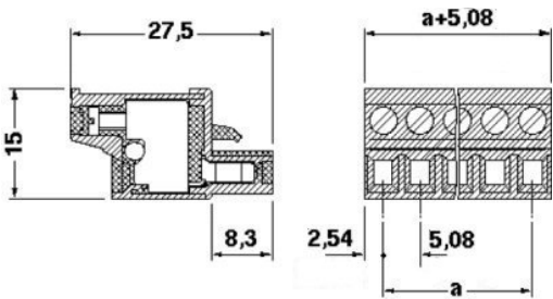
Dimensioned drawing
