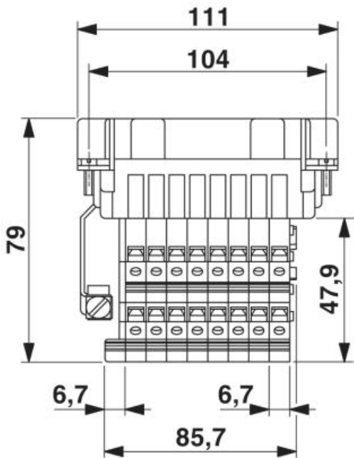
Dimensioned drawing
