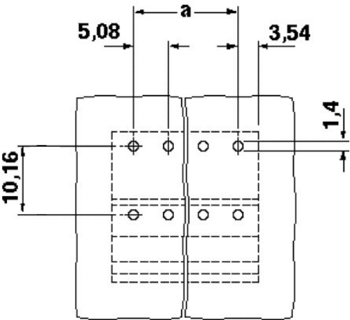
Drilling diagram
