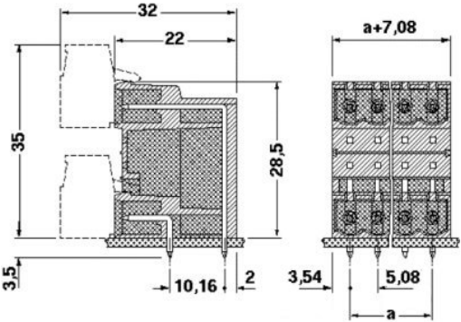
Dimensioned drawing
