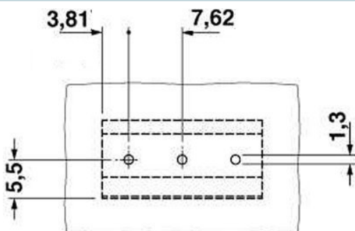
Drilling diagram
