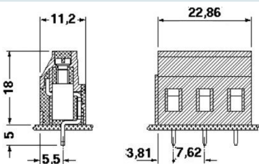
Dimensioned drawing
