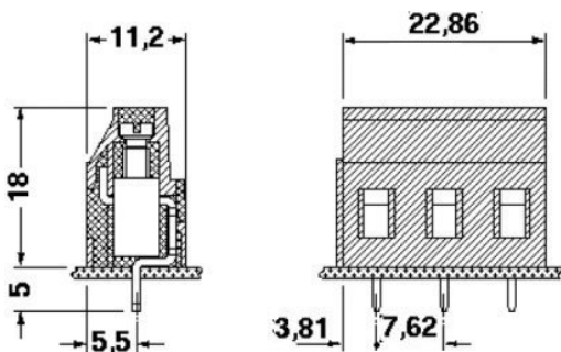
Dimensioned drawing
