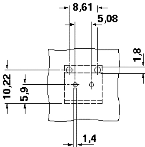
Drilling diagram
