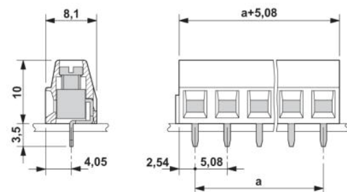
Dimensioned drawing
