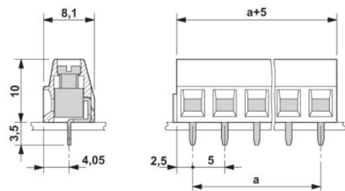
Dimensioned drawing
