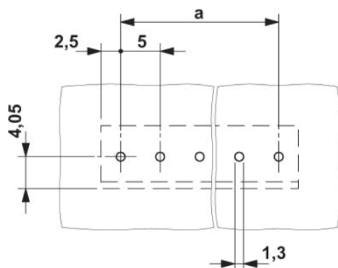
Drilling diagram
