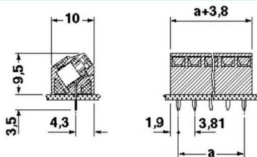
Dimensioned drawing
