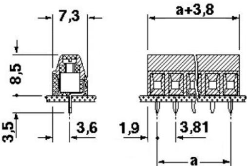
Dimensioned drawing
