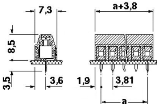
Dimensioned drawing
