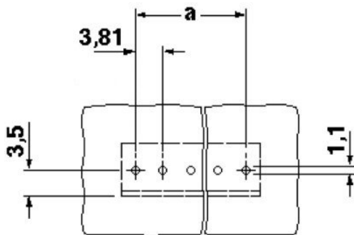
Drilling diagram
