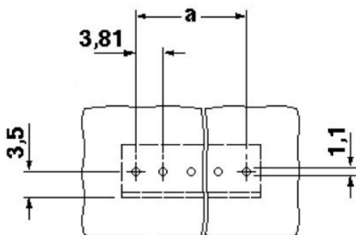
Drilling diagram
