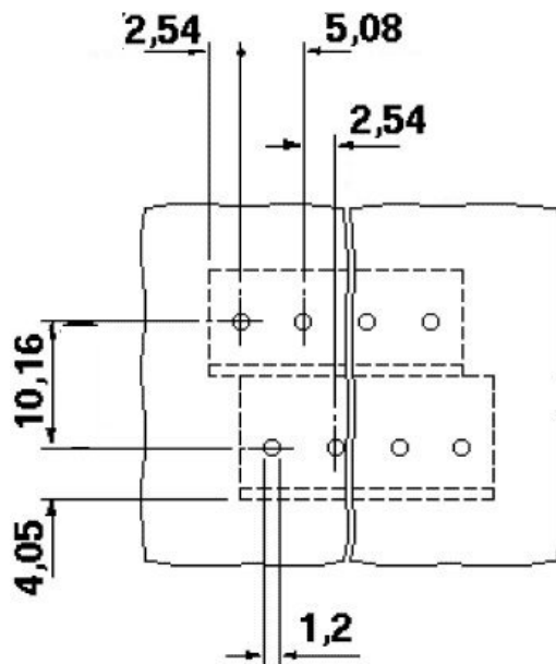
Drilling diagram
