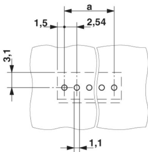
Drilling diagram
