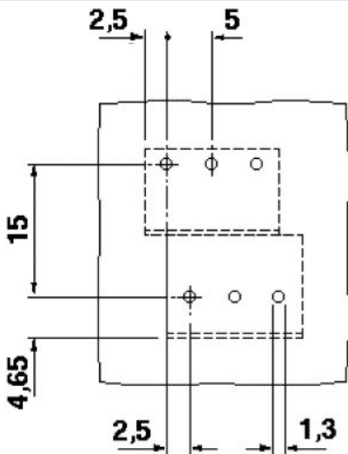
Drilling diagram
