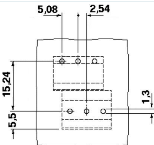
Drilling diagram
