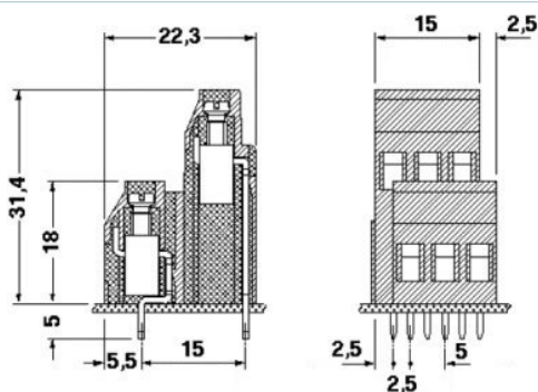
Dimensioned drawing
