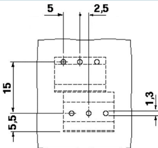
Drilling diagram
