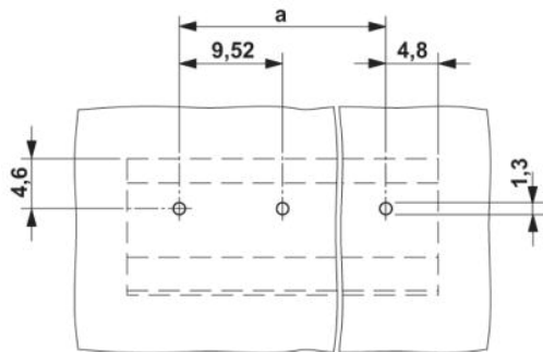
Drilling diagram
