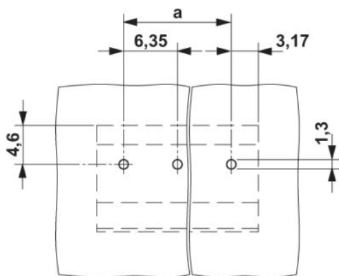
Drilling diagram
