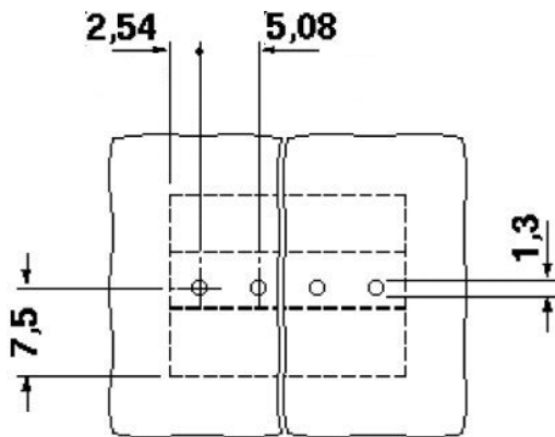
Drilling diagram
