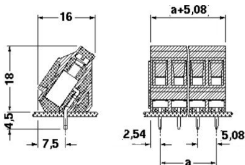
Dimensioned drawing
