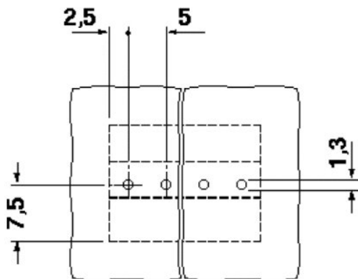
Drilling diagram
