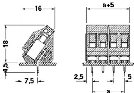
Dimensioned drawing
