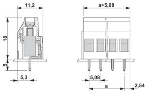
Dimensioned drawing
