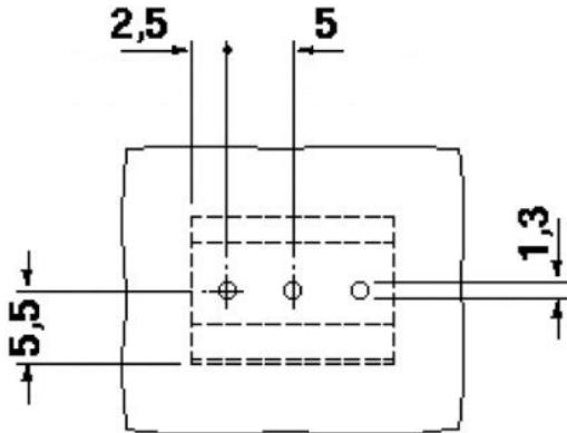
Drilling diagram
