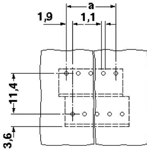
Dimensioned drawing
