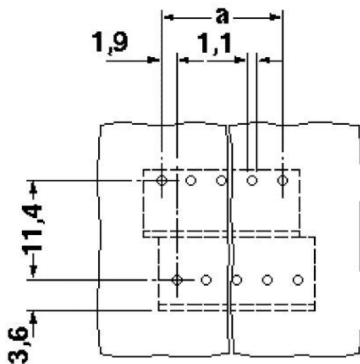
Drilling diagram
