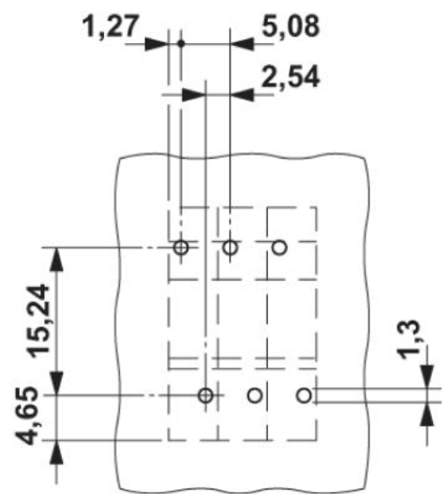
Drilling diagram
