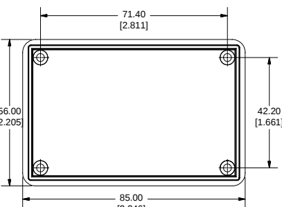
BOTTOM VIEW OF LID
