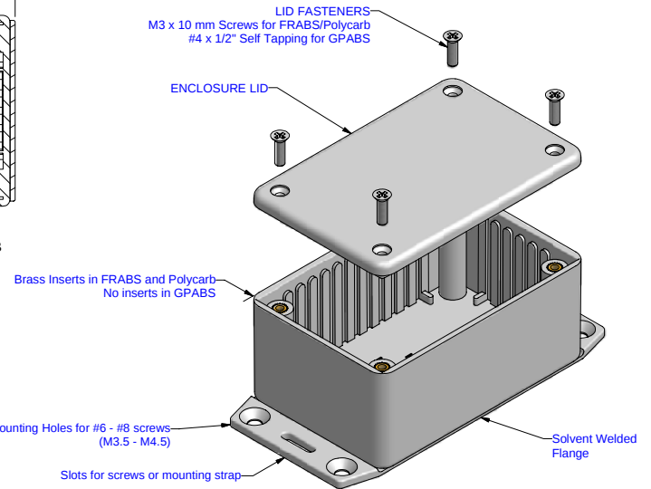
EXPLODED VIEW OF ENCLOSURE
