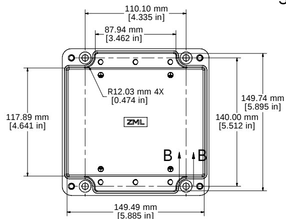
BOX - INSIDE
