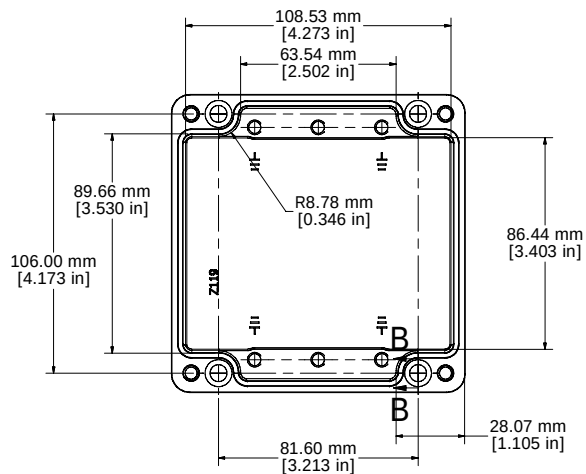
BOX - INSIDE
